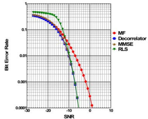
Figure.4a. Bit error rate verses average signal to noise ratio for linear CDMA multi-user standard detectors in linear time invariant channel and SIR=-20dB.
