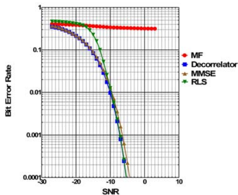
Figure.5a. Bit error rate verses average signal to noise ratio for linear CDMA multi-user standard detectors in linear time invariant channel and SIR=-40dB.
