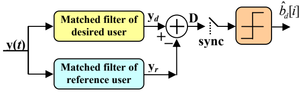
Figure.2. Proposed two signatures decorrelator detector structure.
