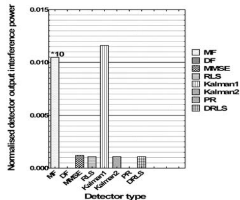
Figure.6. the interference signal power at the output of linear CDMA multi-user standard detectors in linear time invariant channel and SIR=-20dB.
