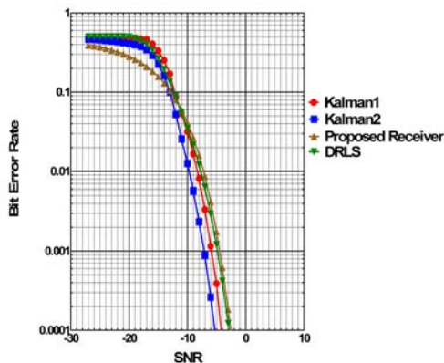
Figure.5b. Bit error rate verses average signal to noise ratio for linear CDMA multi-user standard detectors in linear time invariant channel and SIR=-40dB.
