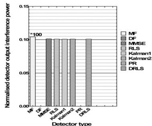
Figure.7. the interference signal power at the output of linear CDMA multi-user standard detectors in linear time invariant channel and SIR=-40dB.
