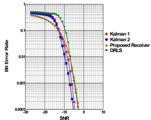
Figure.4b. Bit error rate verses average signal to noise ratio for linear CDMA multi-user standard detectors in linear time invariant channel and SIR=-20dB.
